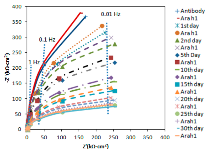
Figure 7. Nyquist plot of the interfacial impedance for the regeneration of Si electrode for 30 days. Test solution contains 50 mM PBS and 5 mM K_3Fe(CN)_6/K_4Fe(CN)_6 at pH 7.3.
